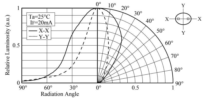
■ Directivity (NSPB636AS)
