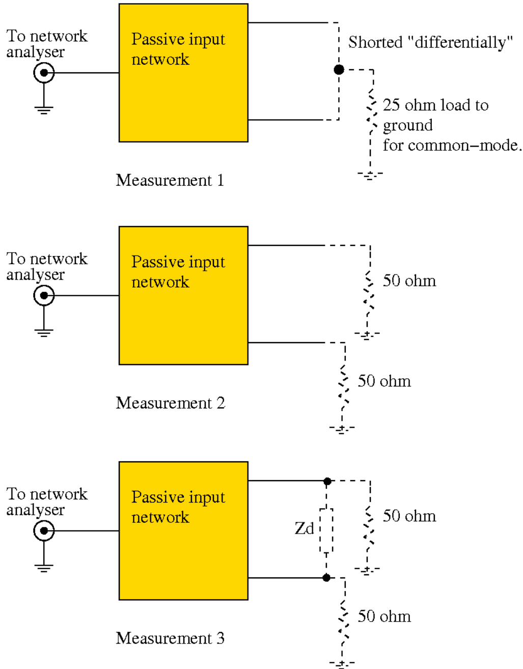
Figure 3: Illustration of measurement setup for extracting equivalent S parameters of input network. The network analyzer connection is unbalanced (single-ended) whereas the loads need to be applied to a balanced line.
