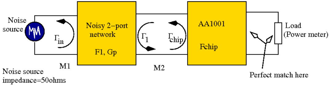
Figure 2: Illustration of cascaded networks that are not necessarily matched.
